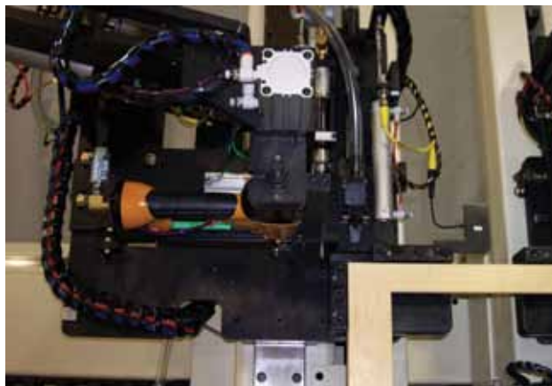
Corner fastening, predrilling and hardware installation.
